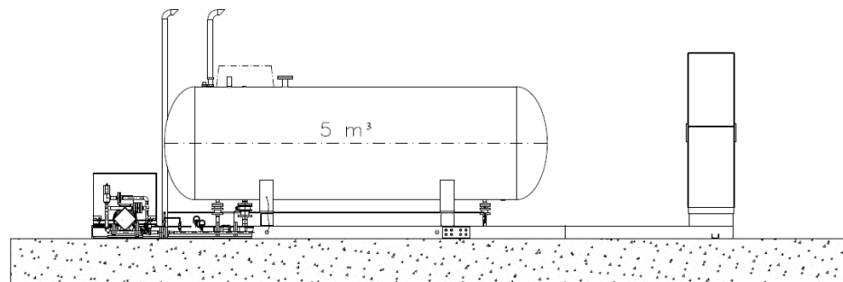
Tip C: Nadzemni SKID s spremnikom 5m 3
